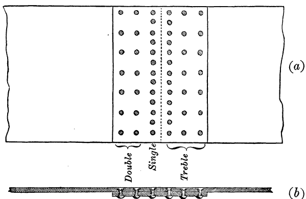
FIG. 51.—Counter-sunk riveting.
