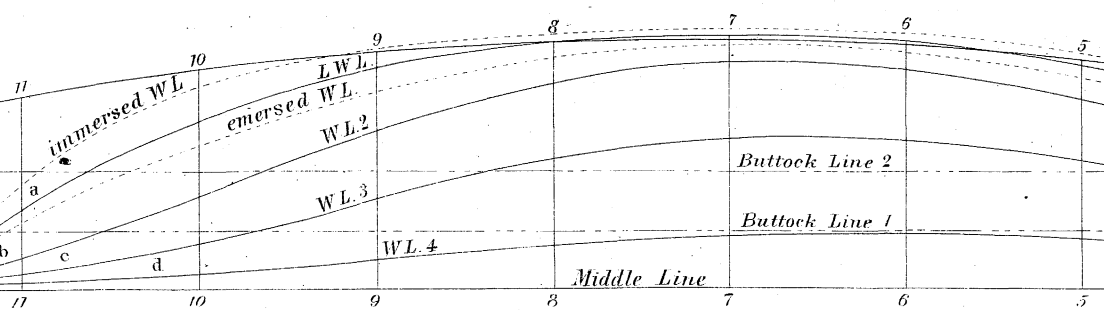
Fig. 28 HALF BREADTH PLAN
