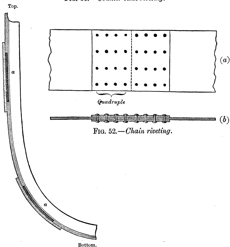
FIG. 53.—Outside and inside plating.
